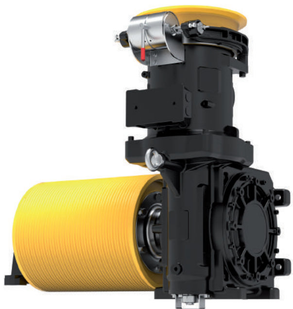
GEARED SH160T
