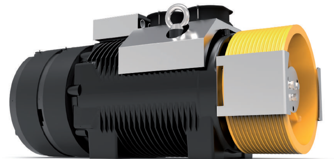
GEARLESS SG75/F
